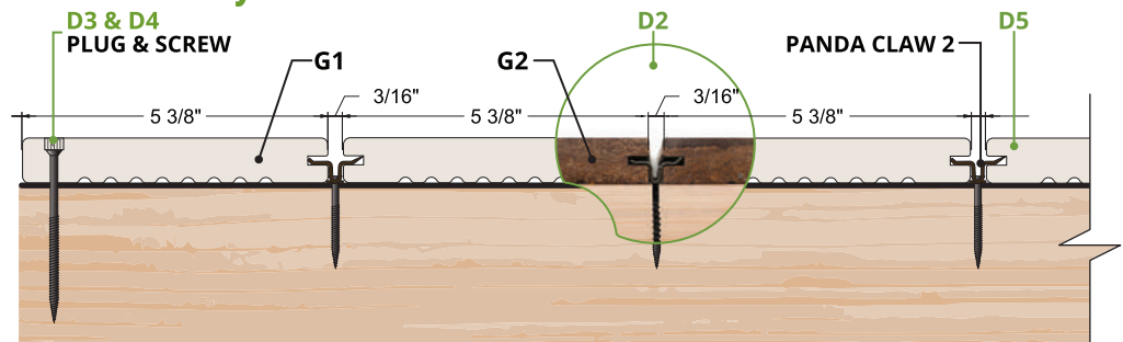
SECTION VIEW
