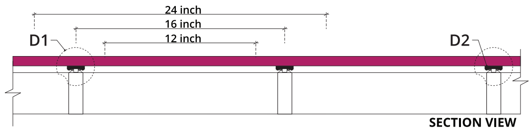
SECTION VIEW
