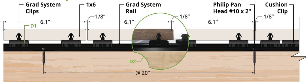
SECTION VIEW
