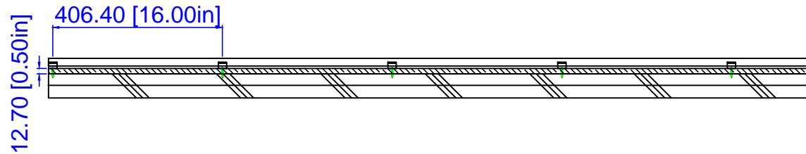
Siding sheathing fastener
