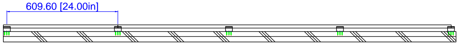
Siding sheathing fastener
