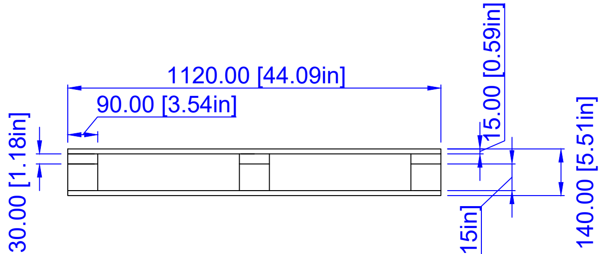
End view
