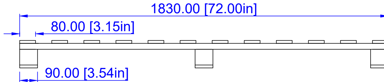
Side view
